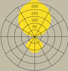
kido 30/46 137lm/W@4000K
