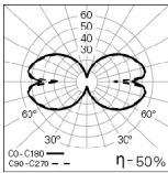
OREO V In Ø970mm bLINE 4000K
