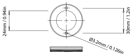
Mounting plate
