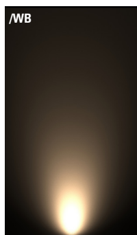
/WB Wide Beam 700mA using a 42° optic
