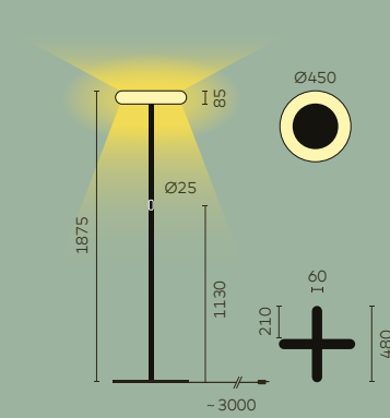
oto standing light
