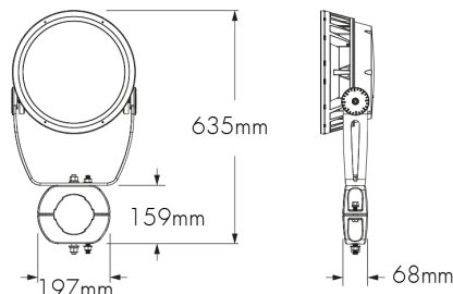
PM4 model shown. Consult factory for square pole section.
