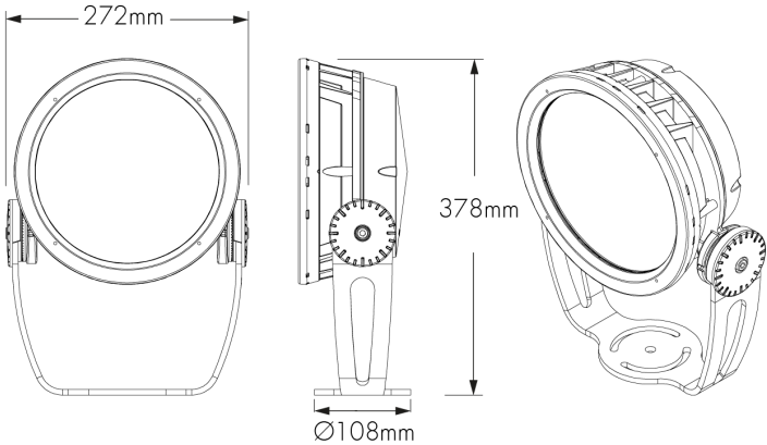
RY - Rotational Yoke
