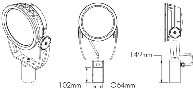
TN2 - Tenon adapter to fit on 60 mm O.D. tenon Vertical mounting only. Consult factory for horizontal mounting.
