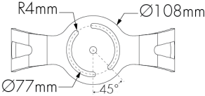
Mounting Hole Pattern - Rotational Yoke
