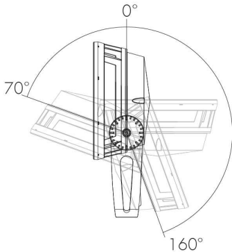
Standard yoke
