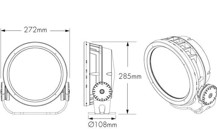
SRY - Short Rotational Yoke
