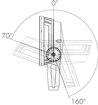
Standard yoke
