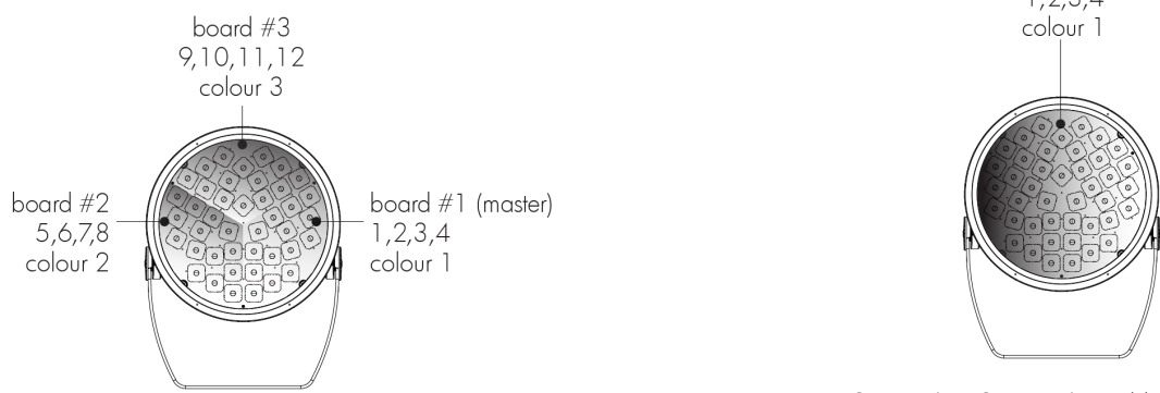
MRGBA and MRGBWP colour mixing options
