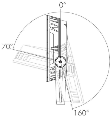
Standard Yoke
