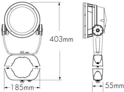
Round Pole Mounting Accessory
