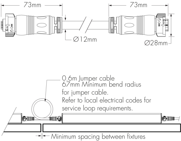
LFJC - Lumenfacade Jumper Cable (XC3P2D)
