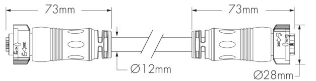
LFJC - Lumenfacade Jumper Cable (XC3P2D)
