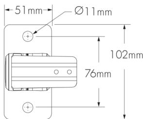
WMCH24 WMIH24 - Mounting Hole Pattern
