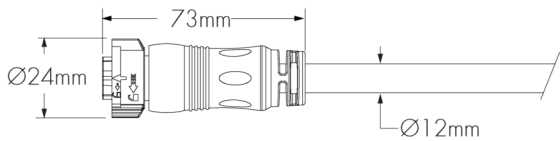
LFCL - Lumenfacade Leader Cable (XC3P3D)
