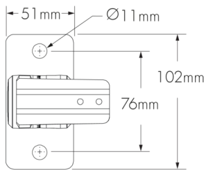
WMCH18 WMIH18 - Mounting Hole Pattern
