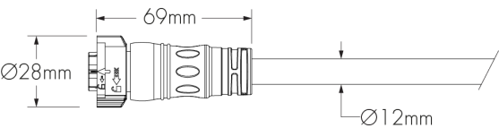
LFLC - Lumenfacade Leader Cable (XC3P2D) 180D (Straight Connector)
