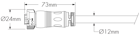
LFLC - Lumenfacade Leader Cable (XC3P3D) 180D (Straight Connector)
