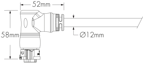
LFLC - Lumenfacade Leader Cable (XC3P2D and XC3P3D) 90D (90° Angle Connector)
