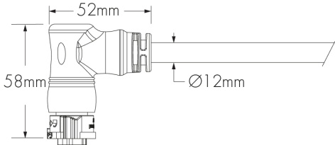
LFCL - Lumenfacade Leader Cable (XC3P2D and XC3P3D) 90D (90° Angle Connector)
