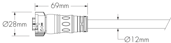
LFCL - Lumenfacade Leader Cable (XC3P2D) 180D (Straight Connector)
