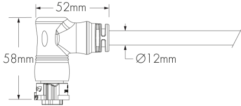
LFCL - Lumenfacade Leader Cable (XC3P2D and XC3P3D) 90D (90° Angle Connector)
