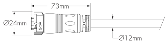
LFCL - Lumenfacade Leader Cable (XC3P3D) 180D (Straight Connector)
