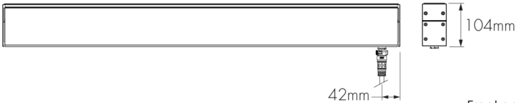
Front and Side Views 913 mm Fixture Shown
