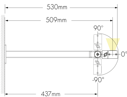
Side-mount installation
