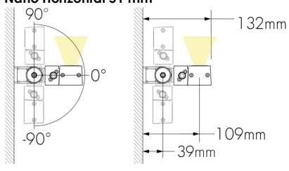
Side-mount installation
