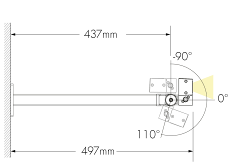
Under-mount installation
