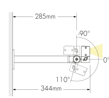
Under-mount installation
