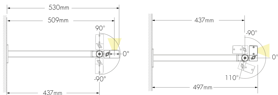
Under-mount installation
