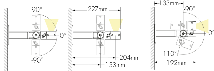
Under-mount installation
