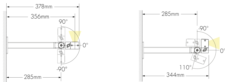
Under-mount installation
