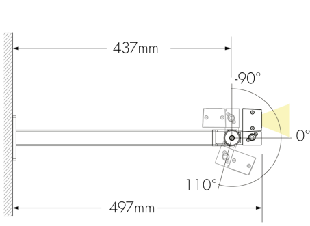
Under-mount installation
