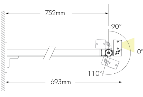
Under-mount installation
