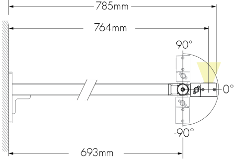
Side-mount installation
