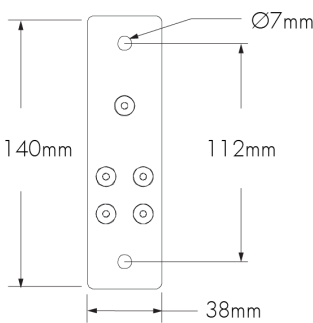
WAMN28 - Mounting Hole Pattern
