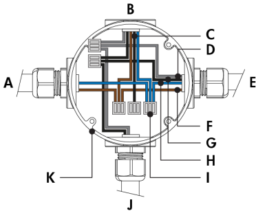
Dim To Warm Via 1-10V (DIM/DTW) - Wiring Detail - CE Class II
