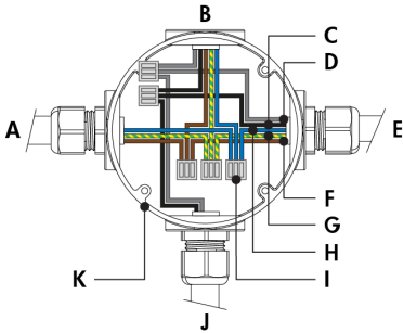
Dim To Warm Via 1-10V (DIM/DTW) - Wiring Detail - CE
