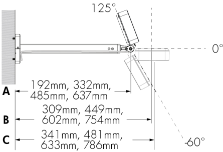
WAM - Wall Mount Bracket With Decorative Cover 152 mm, 305 mm, 457 mm or 610 mm
