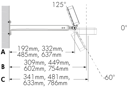
WAMNC - Wall Mount Bracket Without Decorative Cover 152 mm, 305 mm, 457 mm or 610 mm
