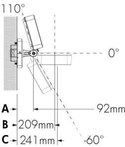
WMRJB - Recessed JBOX Wall Mount With Decorative Cover
