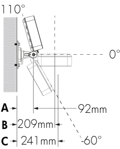
WMNC - Wall Mount Bracket Without Decorative Cover
