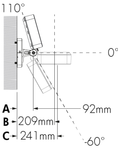
WM - Wall Mount Bracket with Decorative Cover
