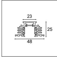
RECESSED PROFILE
