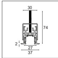
RECESSED FLANGE PROFILE
